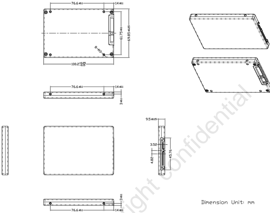
Figure 2: Dimension
